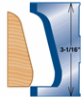
#4526 Casing
