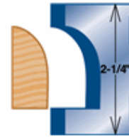
#4523 Shoe Moulding
